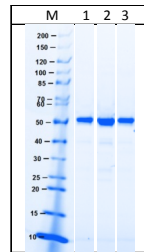
A) SDS-PAGE (reducing conditions) B) SE-HPLC
