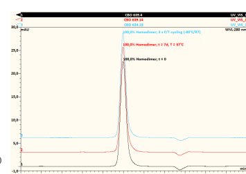
A) SDS-PAGE (reducing conditions) B) SE-HPLC
